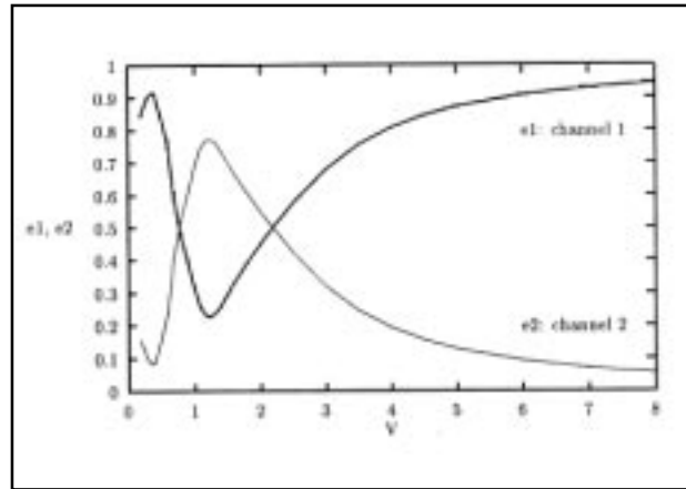
Figure 2.- Relative output probe energies in channels number one and two after soliton collision as function of the collision angle. Other parameters are the same as those in Fig.1.
