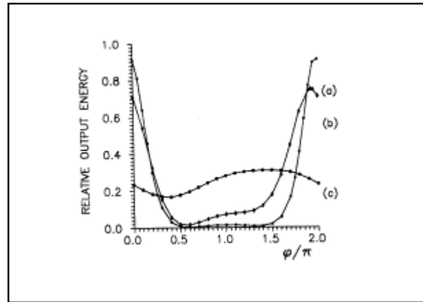
Figure 3.- Relative output probe energy in channel number one as the relative phase between the initial solitons is varied. In (a) \nu=0.375 , in (b) \nu=0.625 and in (c) \nu=1.25 . Other parameters are the same as those in Fig.1.
