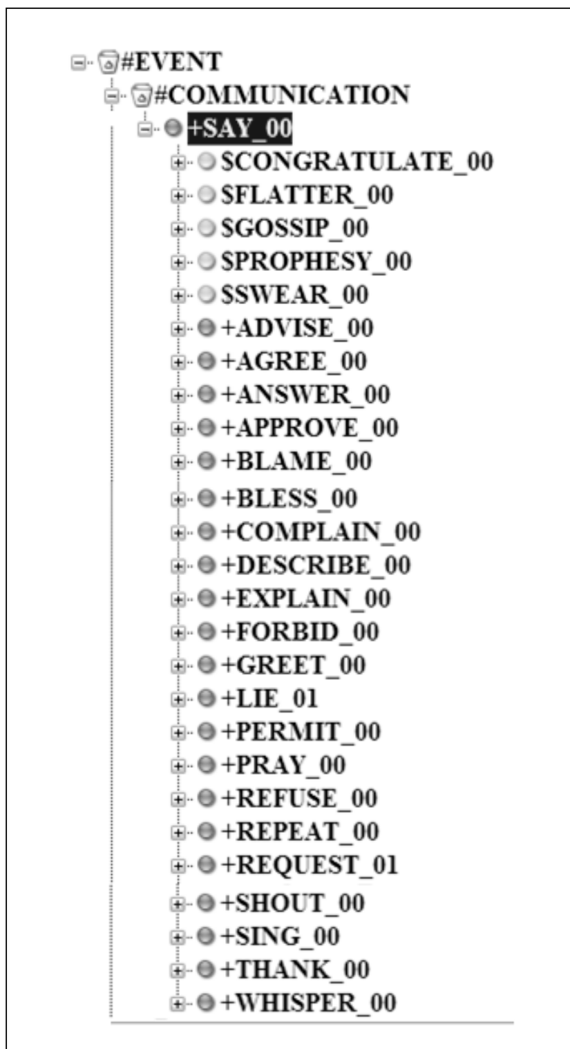
FIGURE 4 The metaconcept #COMMUNICATION in the FunGramKB ontology
