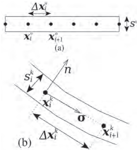
Figure 3. (a) A schematic strip defined by a set of tracers located at x_i for i = 1, \dots, N with a striation thickness s^0 . (b) A section of the strip deformed by the flow after k time steps.
