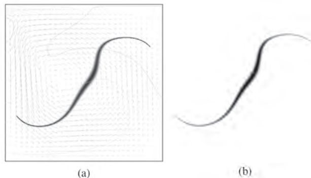
Figure 4. Concentration c displayed on gray levels after 1 cycle of heating-cooling as described in section Natural convection in a square cavity. (a) Result obtained with the CPU version of the algorithm: temperature contours and velocity displayed along the distribution of c . The blue line shows the actual position of the tracers. (b) Result obtained with the real-time visualization algorithm: distribution of c is displayed.
