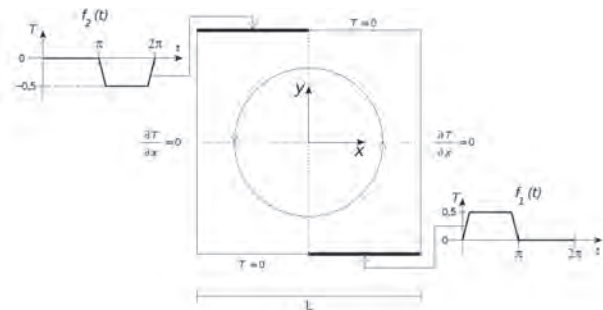
Figure 1. Square cavity geometry and boundary conditions
