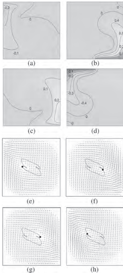
Figure 2. Temperature and velocity fields for: (a) and (e) \phi = 0 ; (b) and (f) \phi = \pi/2 ; (c) and (g) \phi = \pi ; and (d) and (h) \phi = 3\pi/2 . The line is the trajectory of the center of the vortex and the dot is the instantaneous position of the center of the vortex.
