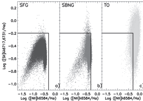
Figure 3: Spectral diagnostic diagram separating AGNs from SFGs (Cozül et al. 1999). The two limits allow identifying galaxies with an excess of emission, which are found mostly in the upper-right part of the diagram.
