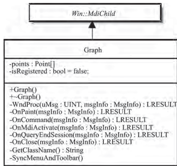
Figure 9. UML diagram showing the Graph class.
