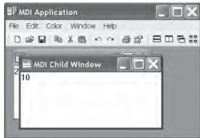
Figure 2. A typical MDI application showing two MDI child windows in cascade mode.
