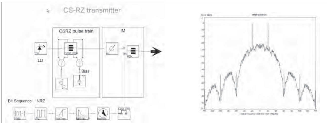
Figure 3. CSRZ transmitter and its spectrum.
