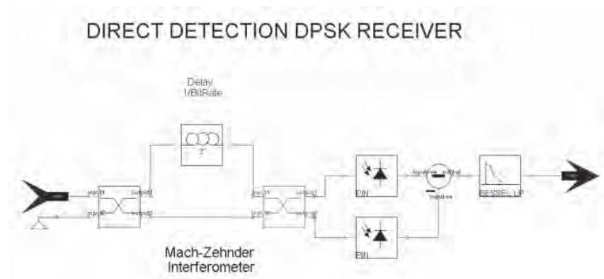
Figure 8. Direct Detection DPSK receiver.
