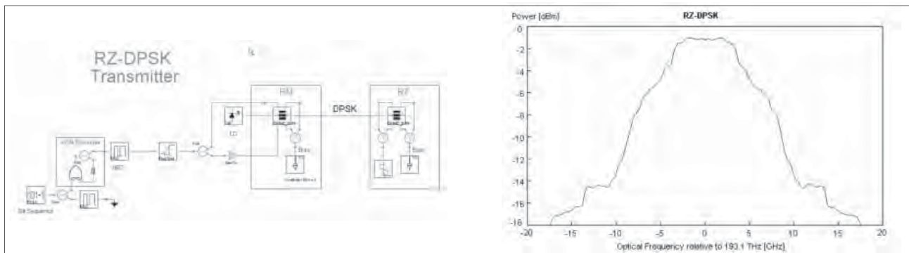
Figure 4. RZ-DPSK transmitter and its spectrum.
