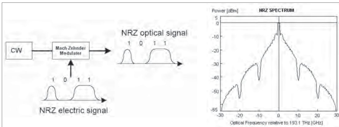
Figure 1. NRZ transmitter diagram and its spectrum.
