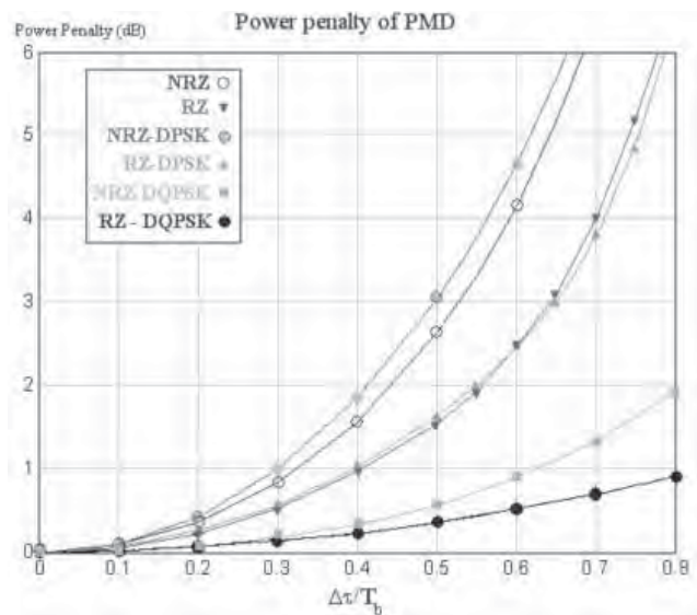
Figure 10. Power Penalty of Polarization Mode Dispersion.
