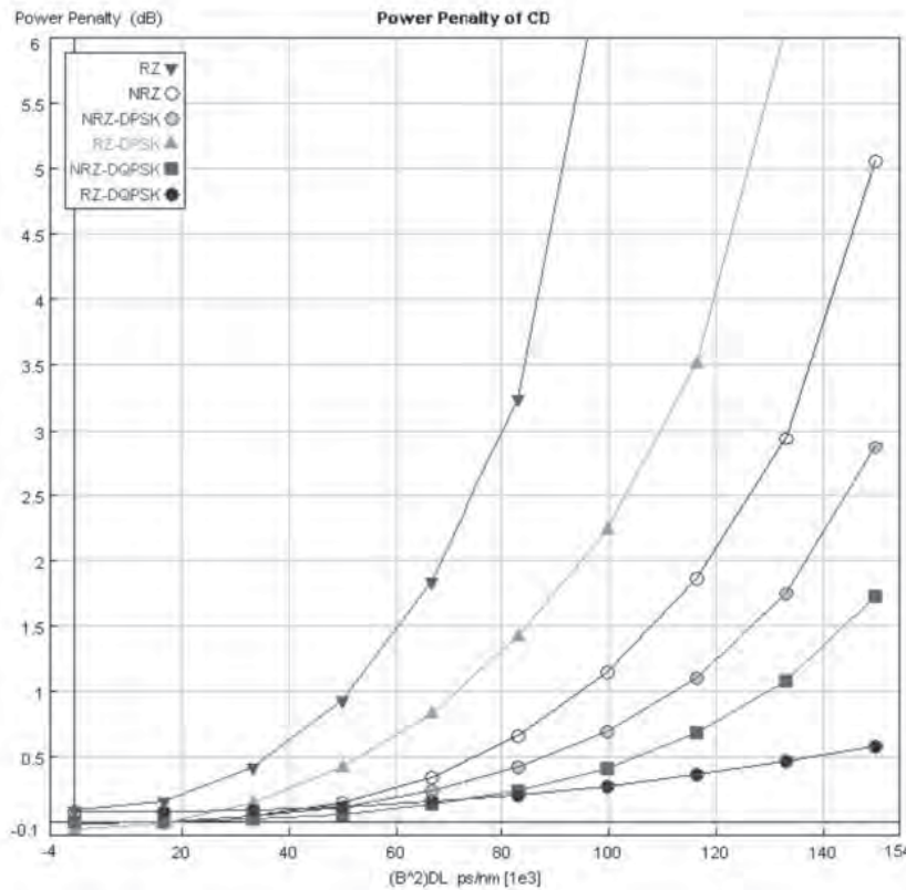
Figure 9. Power Penalty of Chromatic Dispersion.
