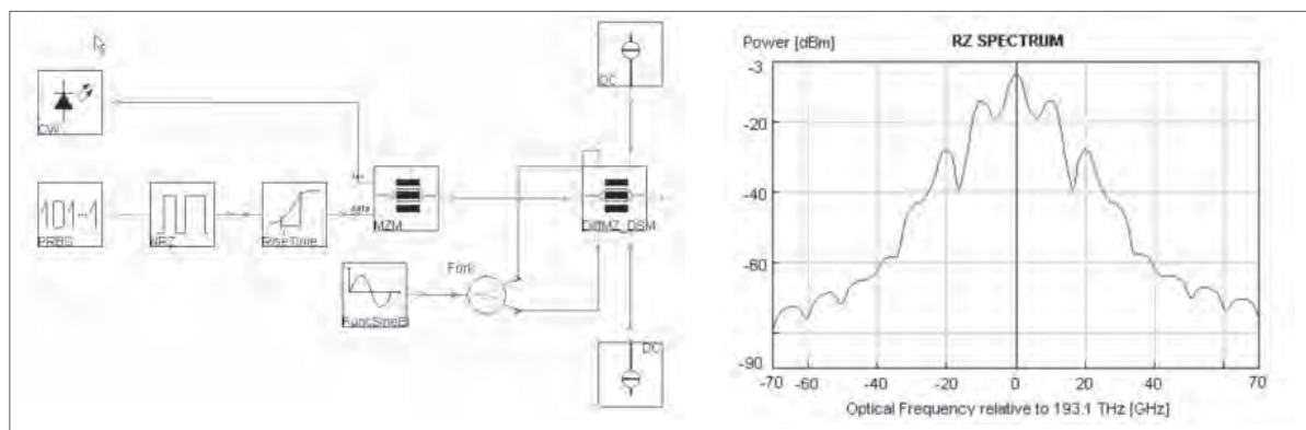
Figure 2. RZ transmitter and its spectrum.
