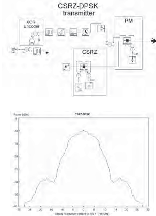
Figure 5. CSRZ-DPSK transmitter and its spectrum.
