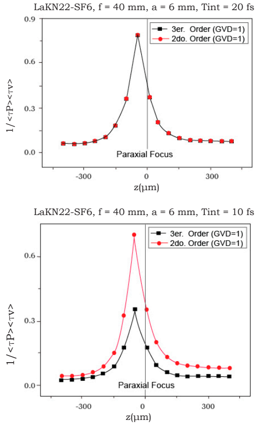
Figure 2. Third order effect of GVD decreases the quality of the signal for pulses of sub-20 fs. Source: Authors own elaboration.
