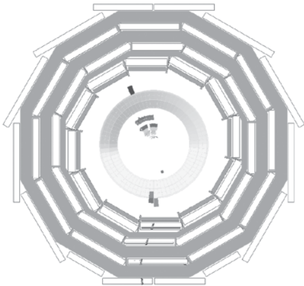
Figure 7. CMS cosmic data event.
