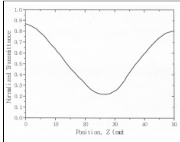
Figure 4. Theoretical fit for the Z-Scan experiment.
